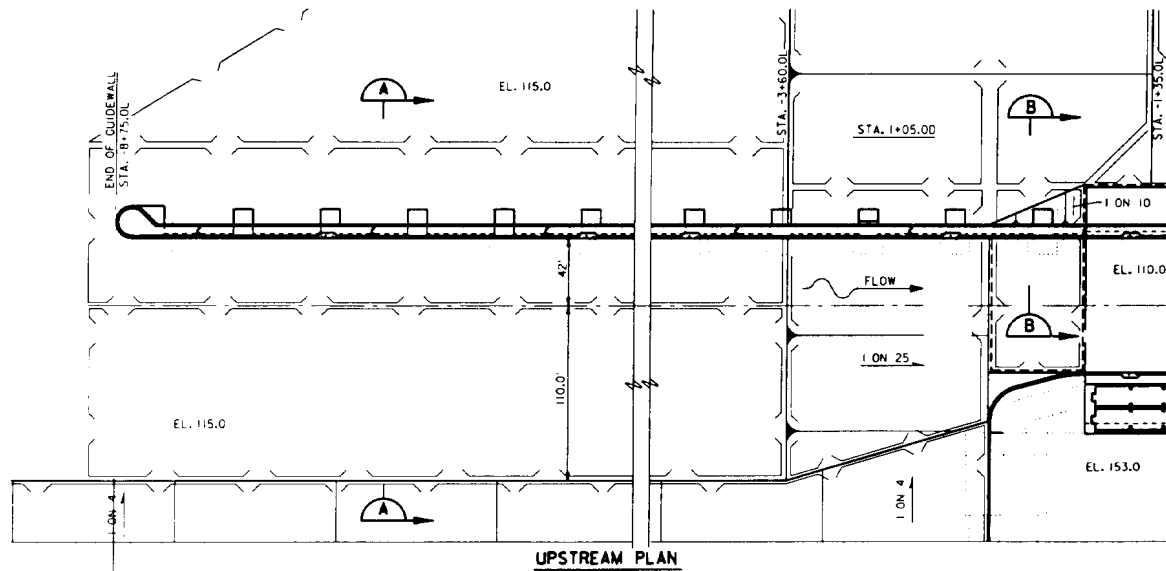
UPSTREAM PLAN
